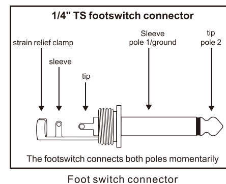
Foot switch connector
