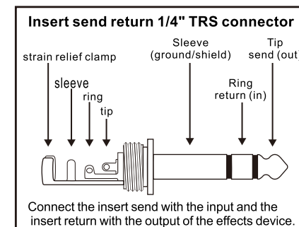
Insert send/return stereo plug
